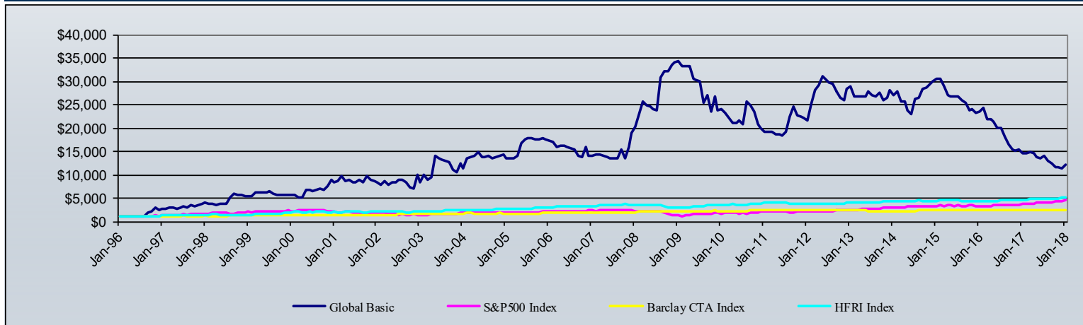
Correlations
